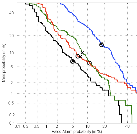
Figure 2: Pooled DET curves of various systems: GMM-SVM (blue), Phone-LM (green), Phone-SVM (red) and the system fusing all of them (black), on the closed-set evaluation subset of 30-second speech segments. Operation points corresponding to actual (X) and minimum (O) C_{avg} are marked on the curves.
